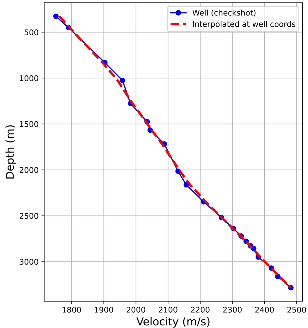
Depth vs Velocity
