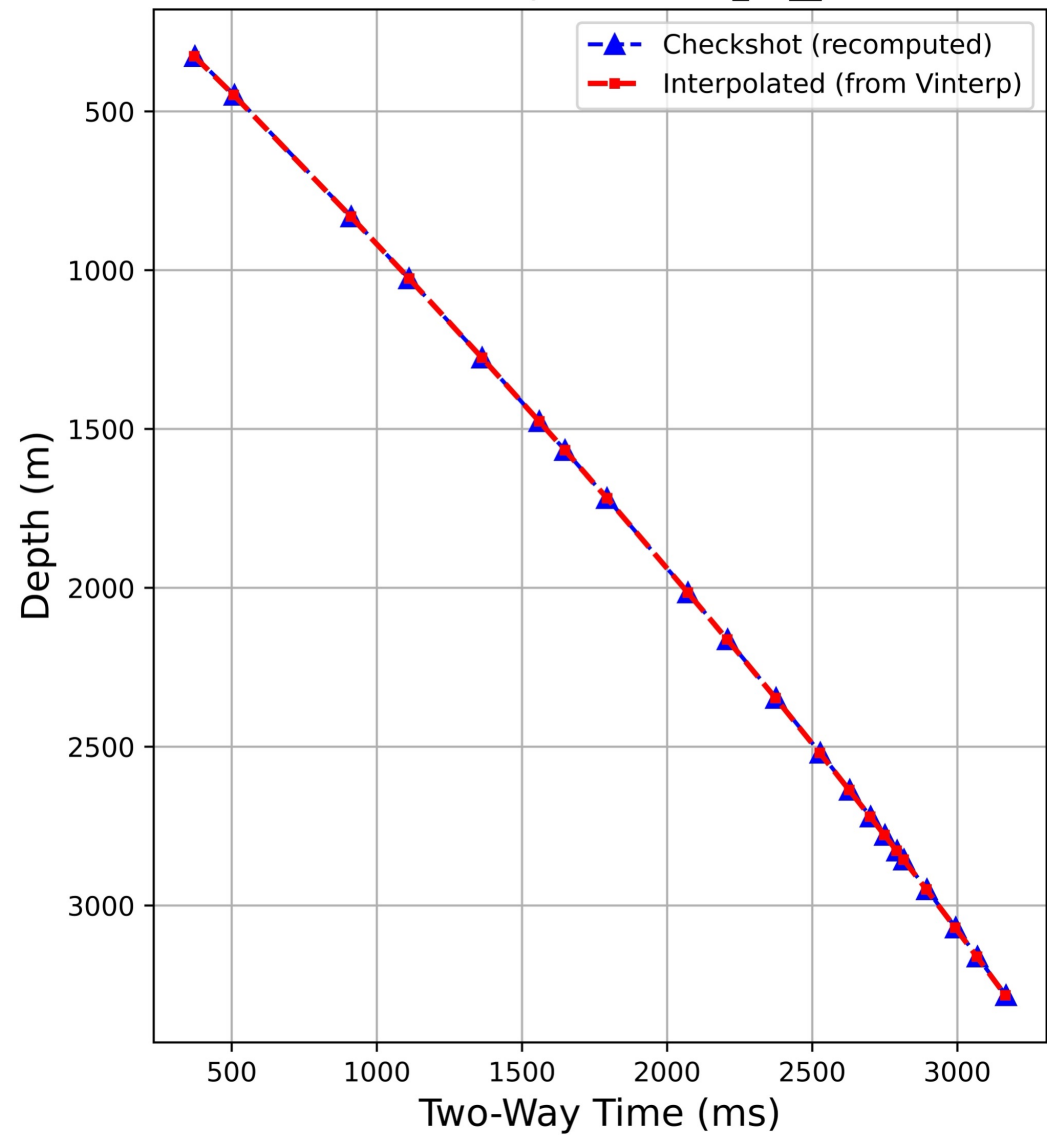
TWT vs Depth at Well 9_12__1
