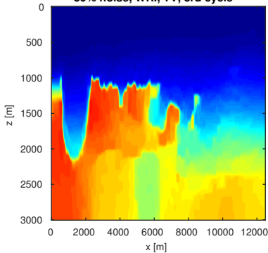
50% noise, WRI, TV, 3rd cycle
