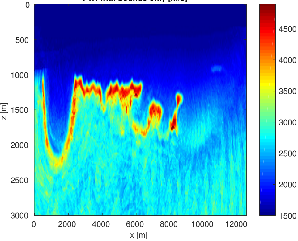
FWI with bounds only [m/s]
