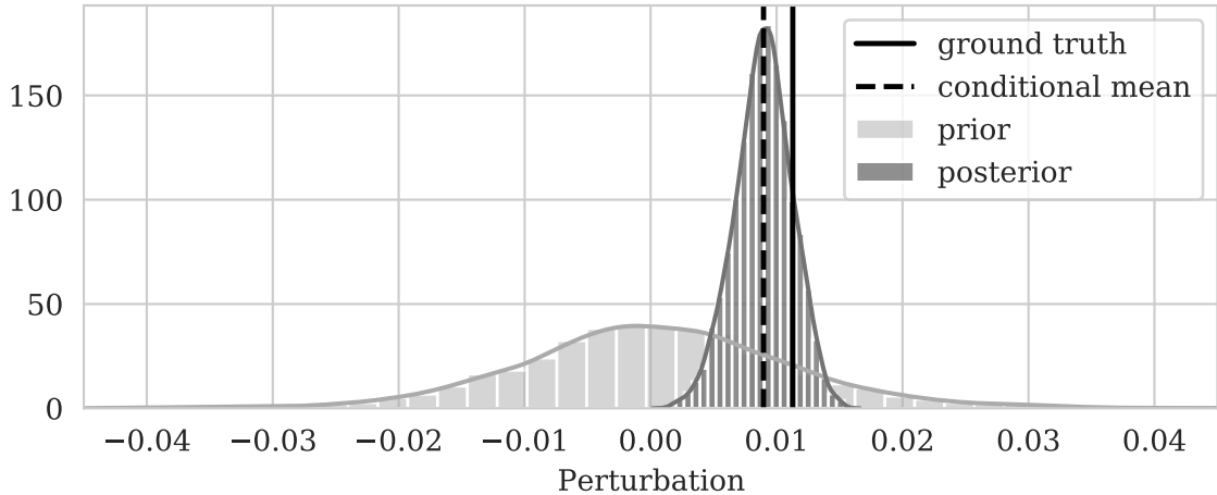
Pointwise histograms at (4.550 km, 1.738 km)
