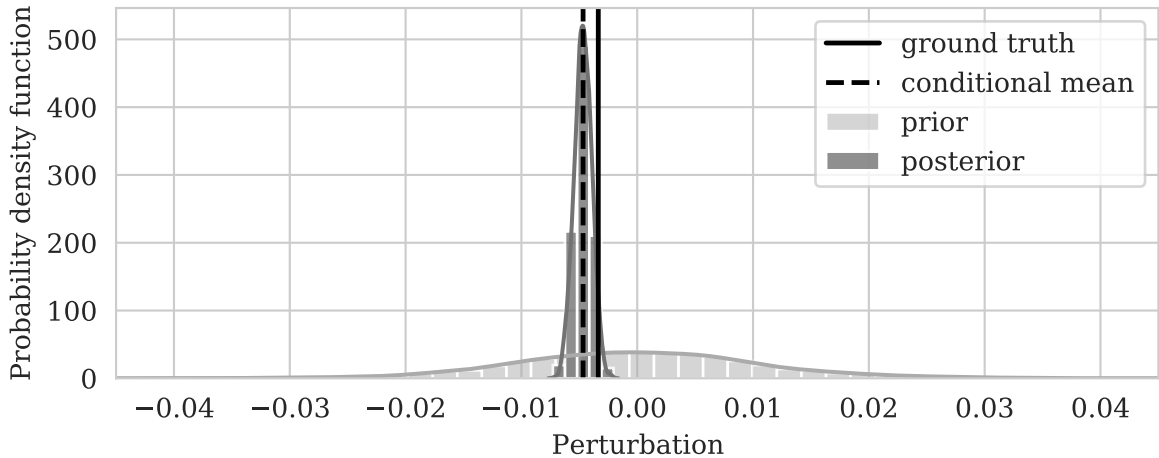
Pointwise histograms at (0.725 km, 0.312 km)
