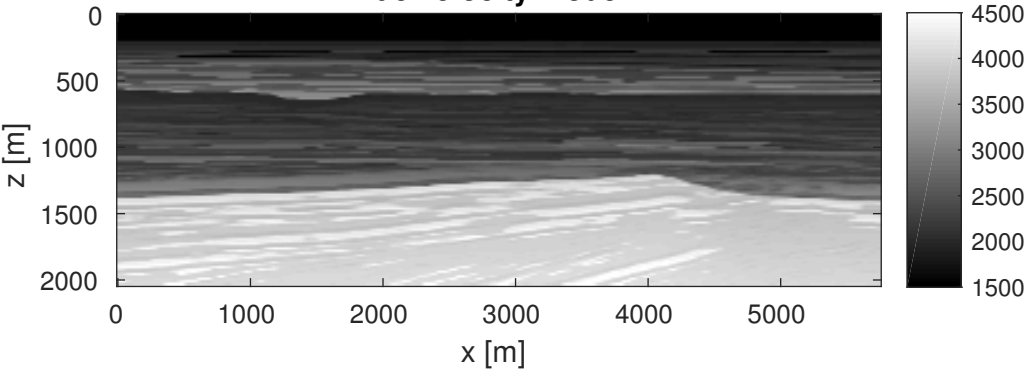
True velocity model
