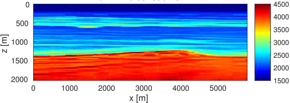
Rank = 10 constraint
