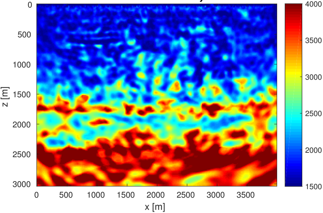
bound constraints only
