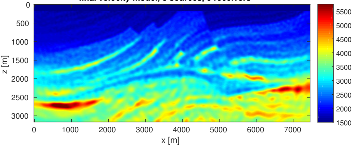
final velocity model, 8 sources, 8 receivers
