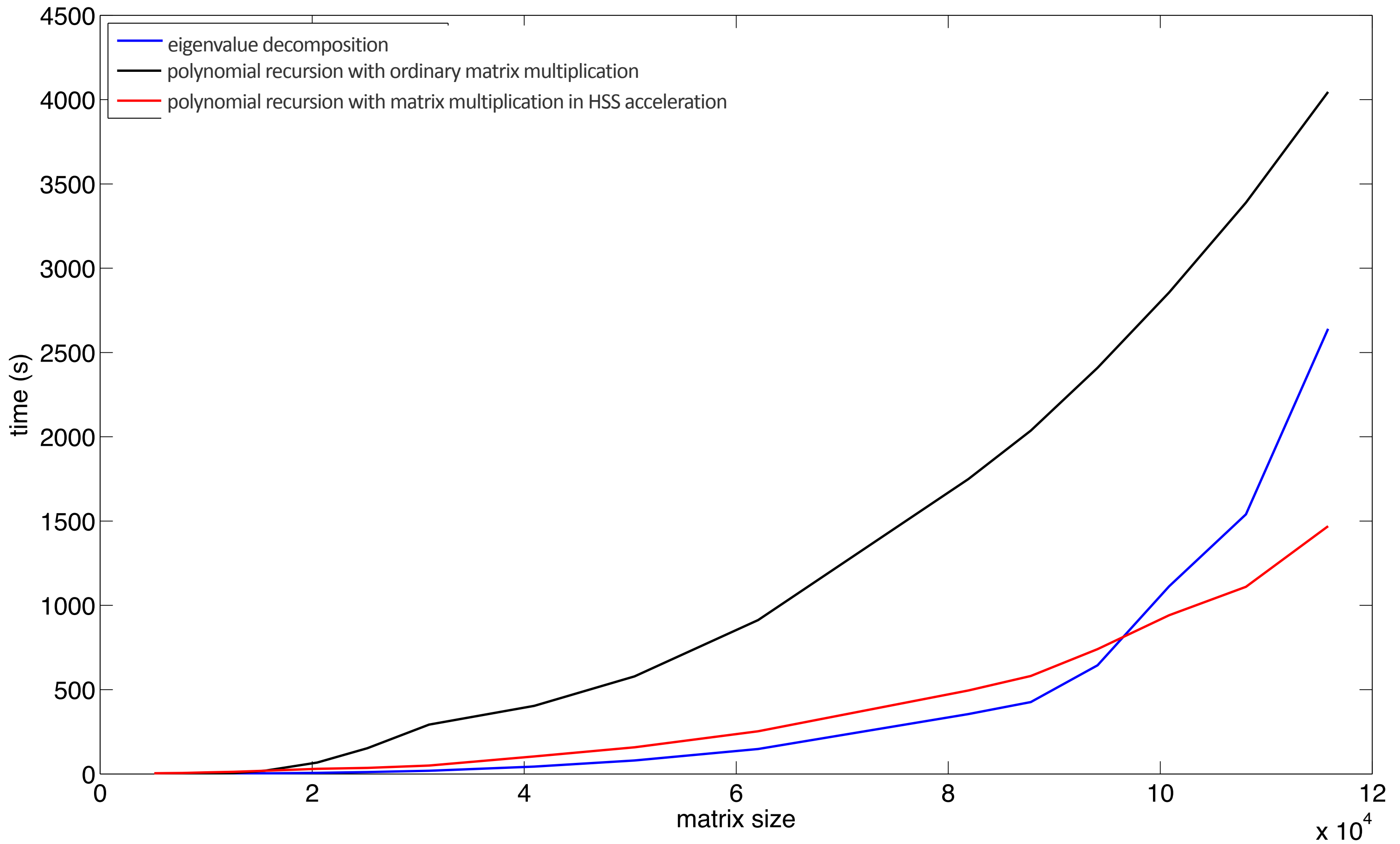
Computation Cost of Spectral Projector
