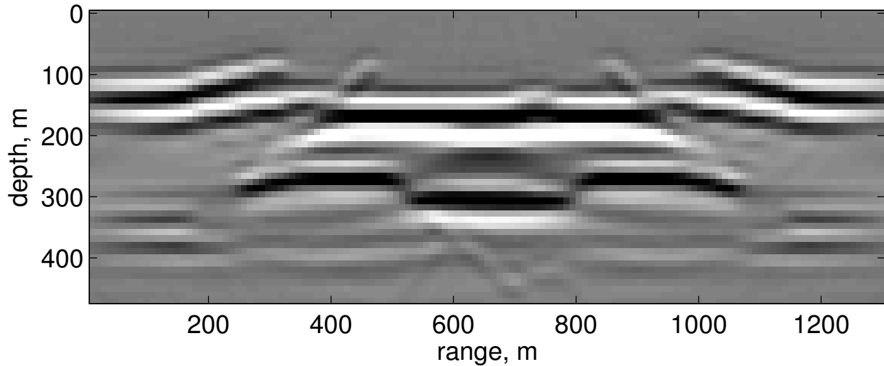
(c) Depth stepping migration
