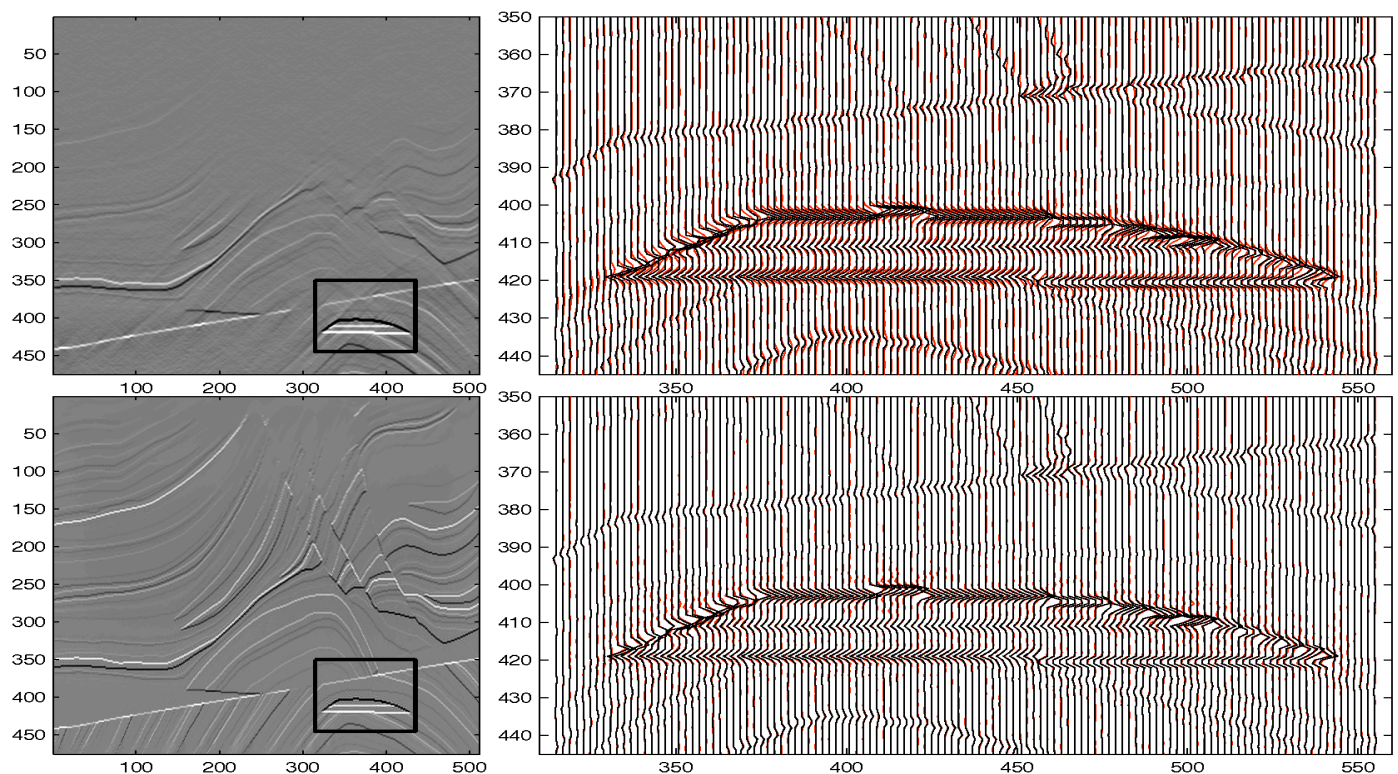
Figure 3. Results for non-convex optimization. (a) Migrated Image, Mean Square Error (MSE): 3.12e6 (b) Enhanced Image, MSE: 3.95e4. Notice the fact that the wiggles at the target zone (black box) of the original and imaged reflectivity more or less overlap for the image created with our optimization method.
